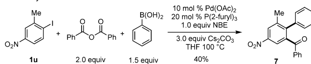
Scheme 2. Coupling with ipso functionalization.
